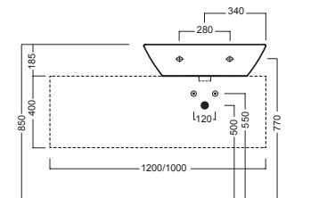
SLIDING wood system_taglio 1 dx - cut 1 rh
